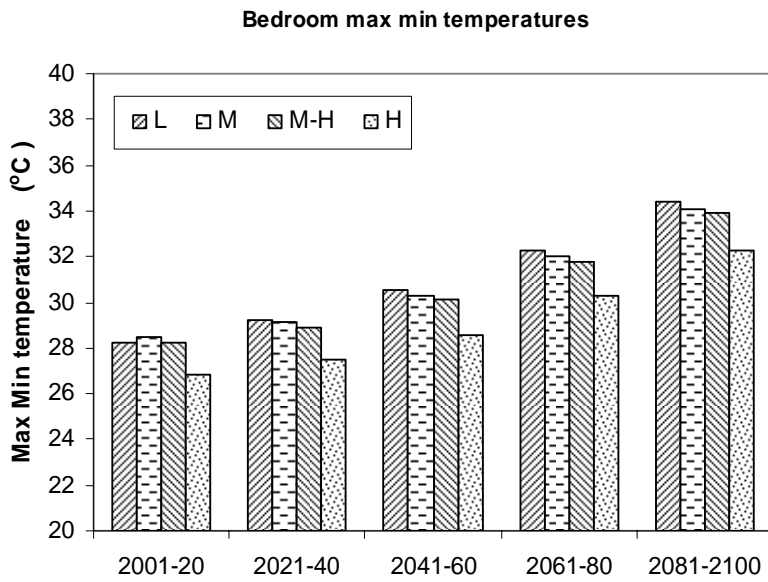
Figure 3: Diagnostics of overheating for the living room and bedrooms, for each 20-year period: (c)&(d): maximum predicted living room operative temperature in the living room and highest night time minimum temperature in the bedrooms.
