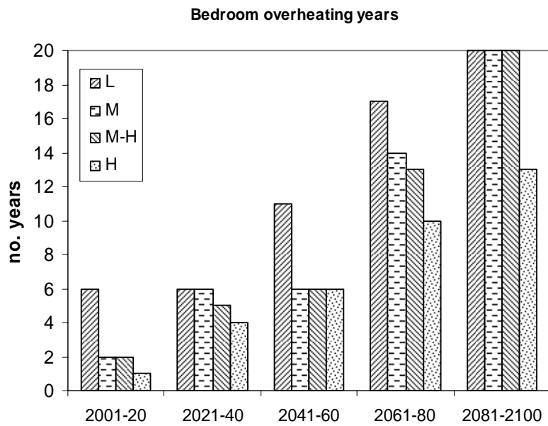
Figure 3: Diagnostics of overheating for the living room and bedrooms, for each 20-year period: (e)&(f): number of years failing the overheating criteria in each 20-year period.
