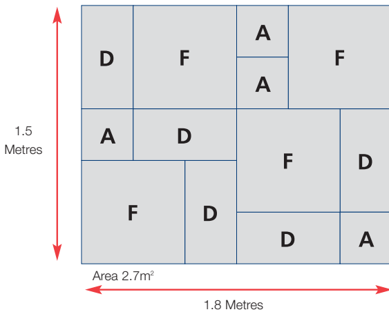
Typical Laying Pattern 3 (Albany, Southwold & Wroxham)
