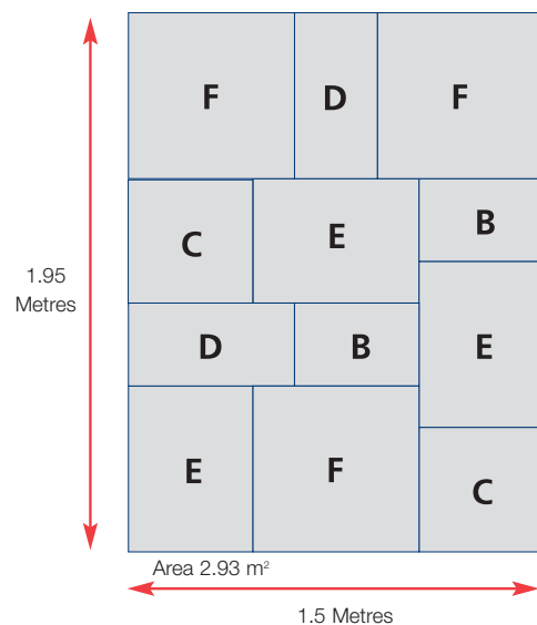
Typical Laying Pattern 4 (Southwold & Wroxham)
