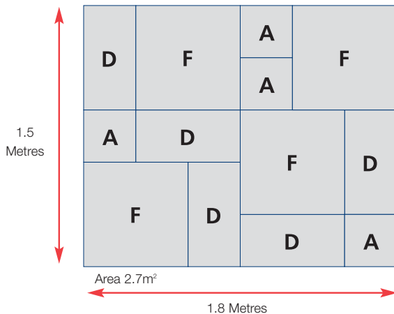
Typical Laying Pattern 3 (Albany, Southwold & Wroxham)
